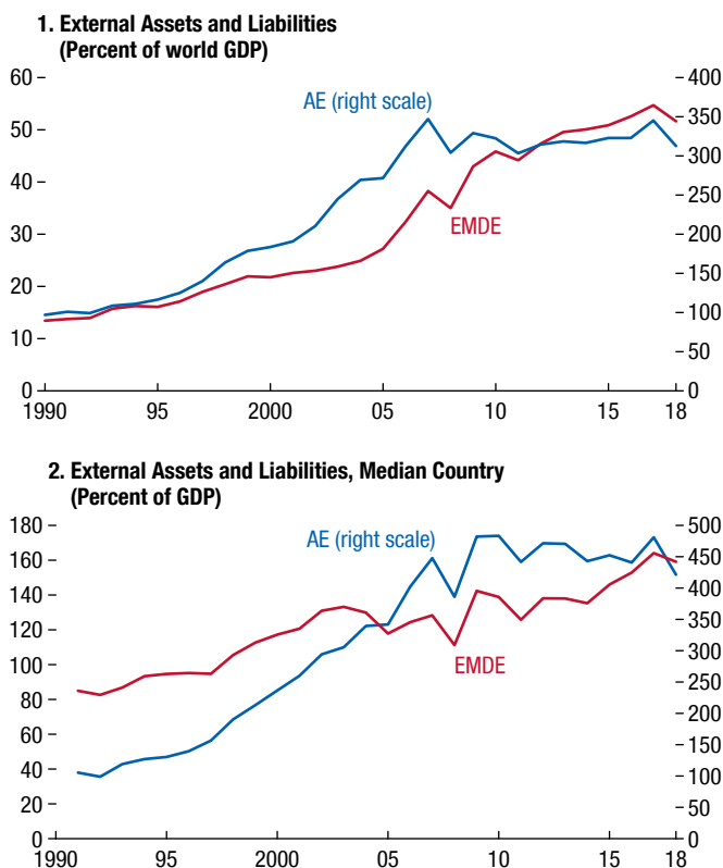
Figure 2.1. Stock Imbalances, 1990–2018
